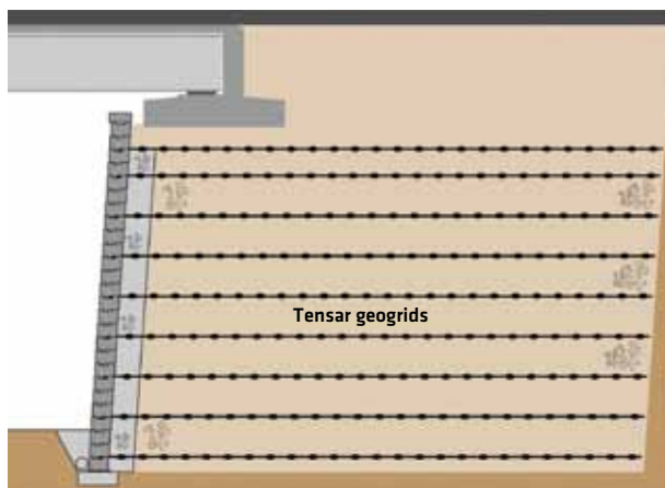
A typical section through a Tensar load bearing bridge abutment detailed here with a modular block facing.
